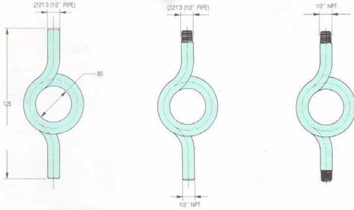
LPP: Welded ends
