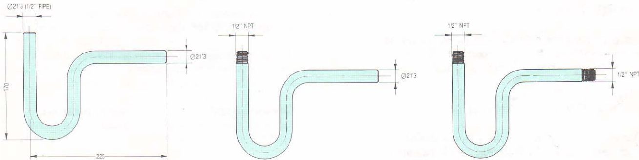
UPP: Welded ends
